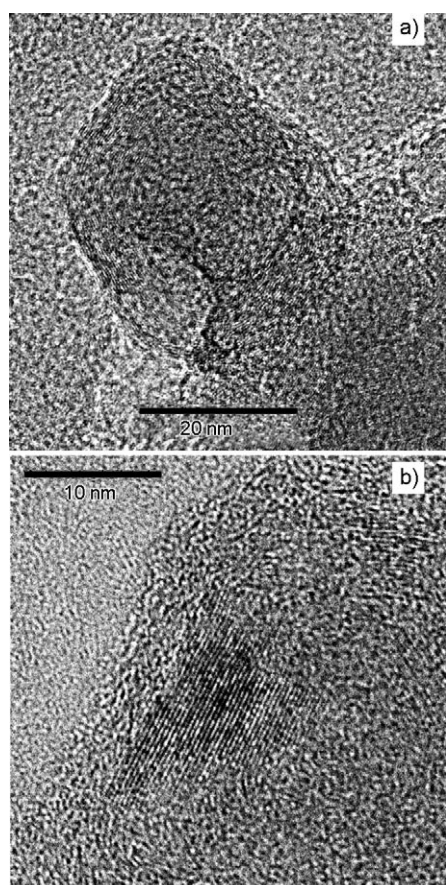
Figure 2. TEM images of \text{K}'_x\text{Ni}^{\text{II}}_y[\text{Fe}^{\text{III}}(\text{CN})_6] Prussian-blue nanoparticles forming into a) disk and b) small rod structures at low concentration (0.05 mol %).
